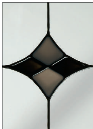
Laptev - Black, Blue, Green & Red
